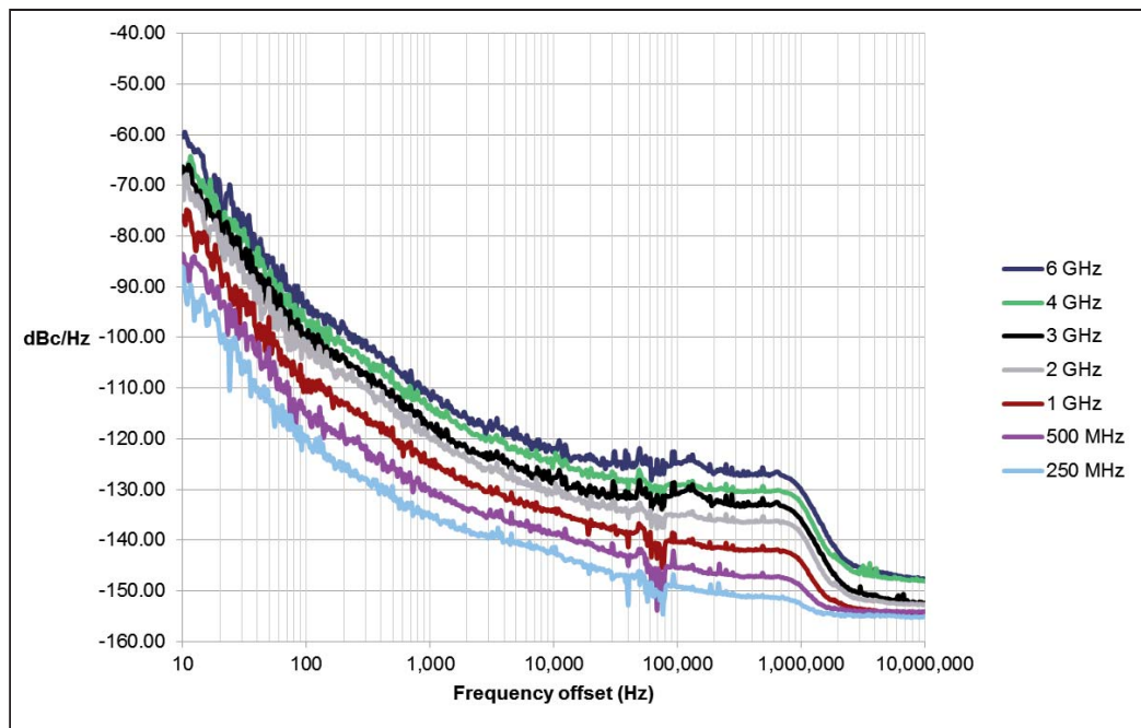
Graph of typical phase noise performance
