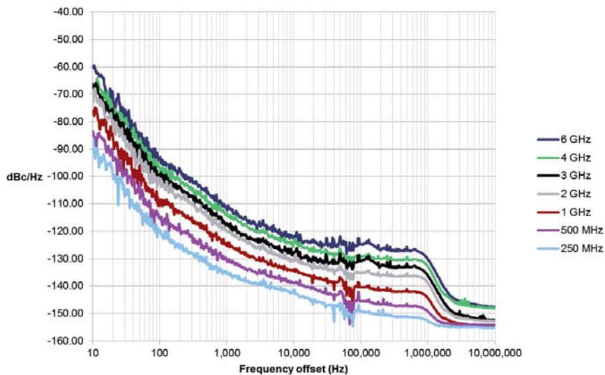
Typical phase noise performance at 250 MHz, 500 MHz, 1 GHz, 2 GHz, 3 GHz, 4 GHz and 6 GHz
