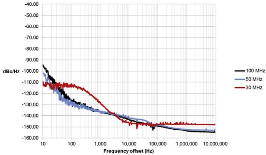
Typical phase noise performance at 30 MHz, 50 MHz and 100 MHz
